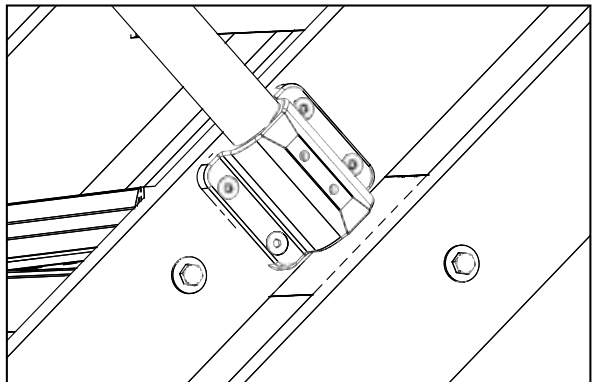
Detail drawing of the rail holders:
