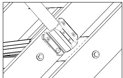
Detail drawing of the holder:
